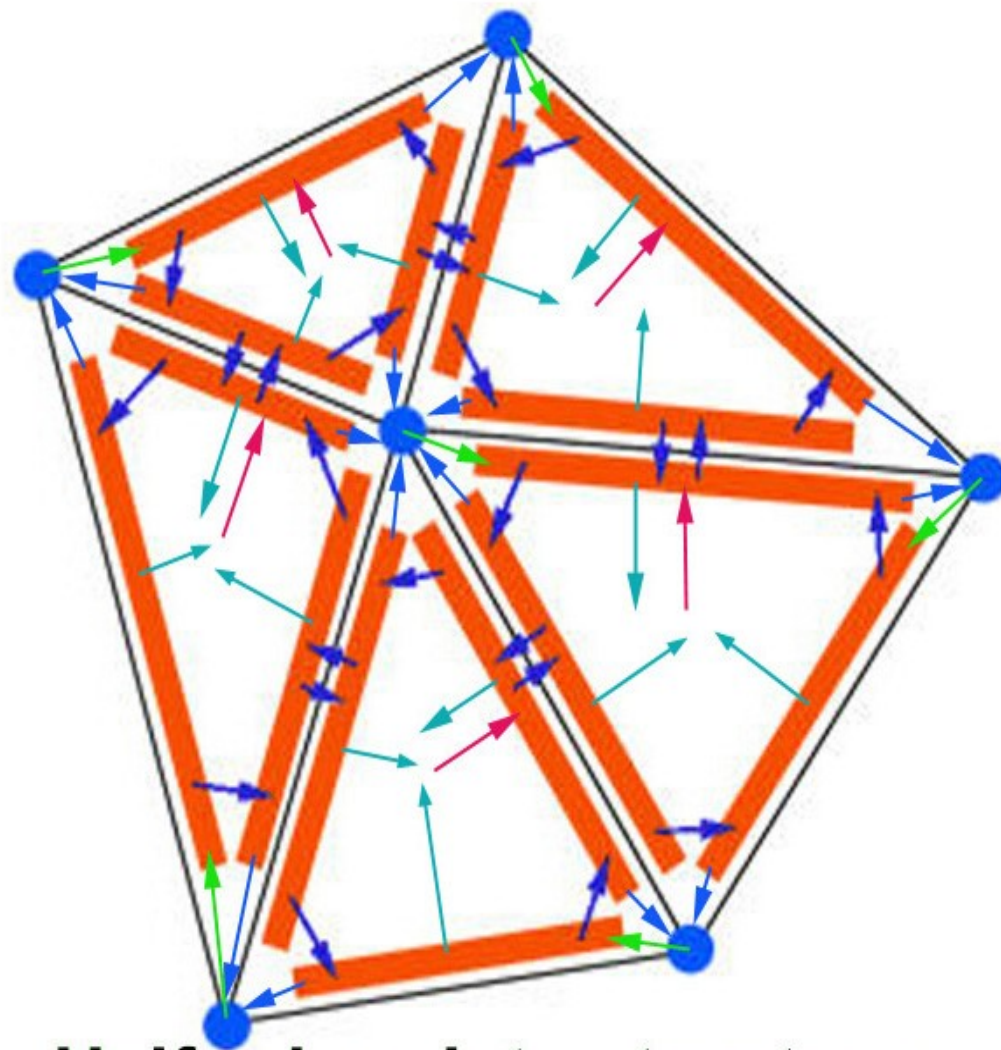
Half-edge data structure
